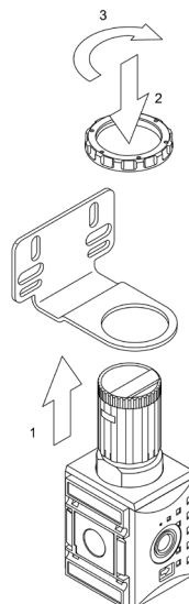
Mounting Plate
